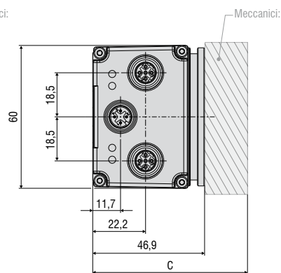
Uscita PN/ENIP/CAT
